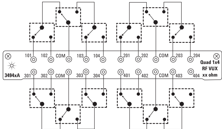
Figure 25. 34941A quad 1*4 50 ohm 3 GHz multiplexer.
