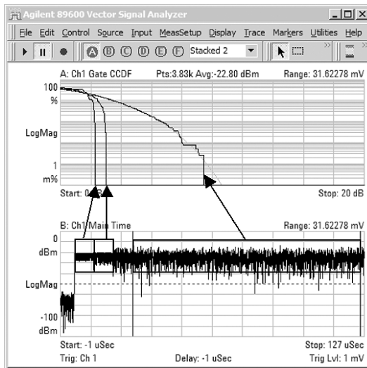
Figure 16. Variations in CCDF during a WLAN packet.
