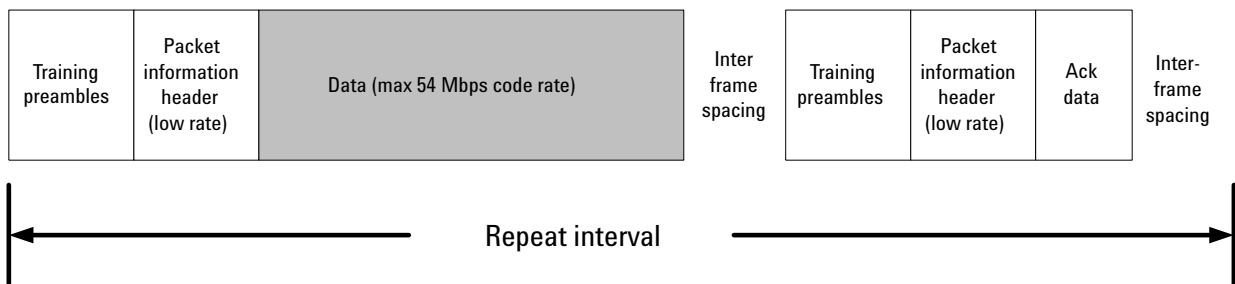
Figure 1. Simplified WLAN OFDM packet timing.
