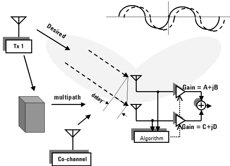
Figure 13. Phased array receiver antenna.
