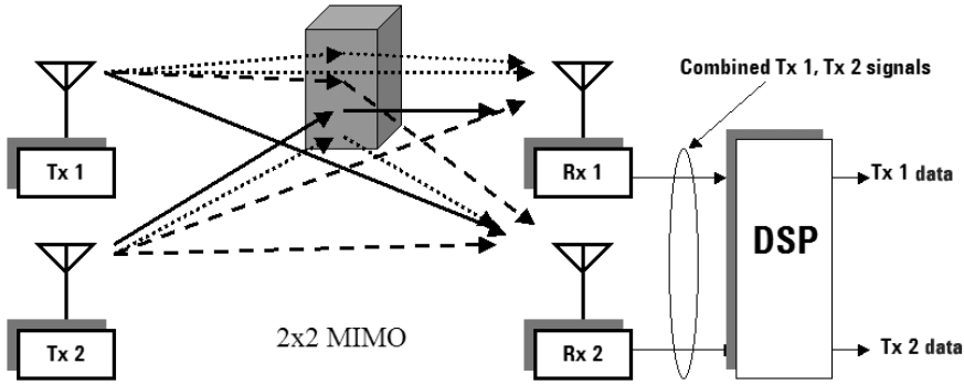
Figure 12. Simplified representation of 2*2 SDM MIMO radio system.
