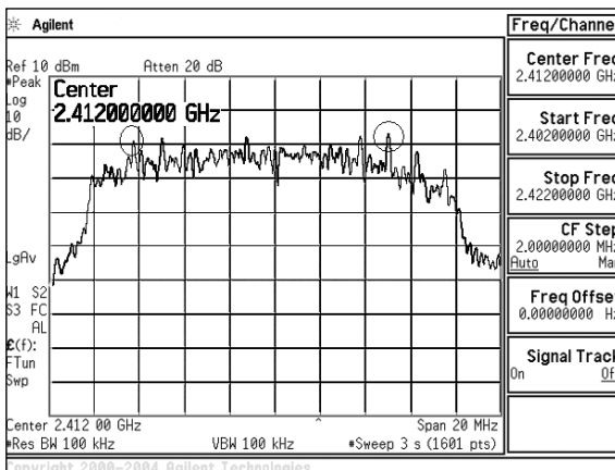
Figure 17. Peaks in power spectrum density measurement accentuated by interaction between antennas.
